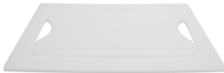
ST11209111EV Strata Rectangular Carving/Display Tray Fits ST11602112 22.5" L x 14.5" W x 0.5" H 1 ea.
